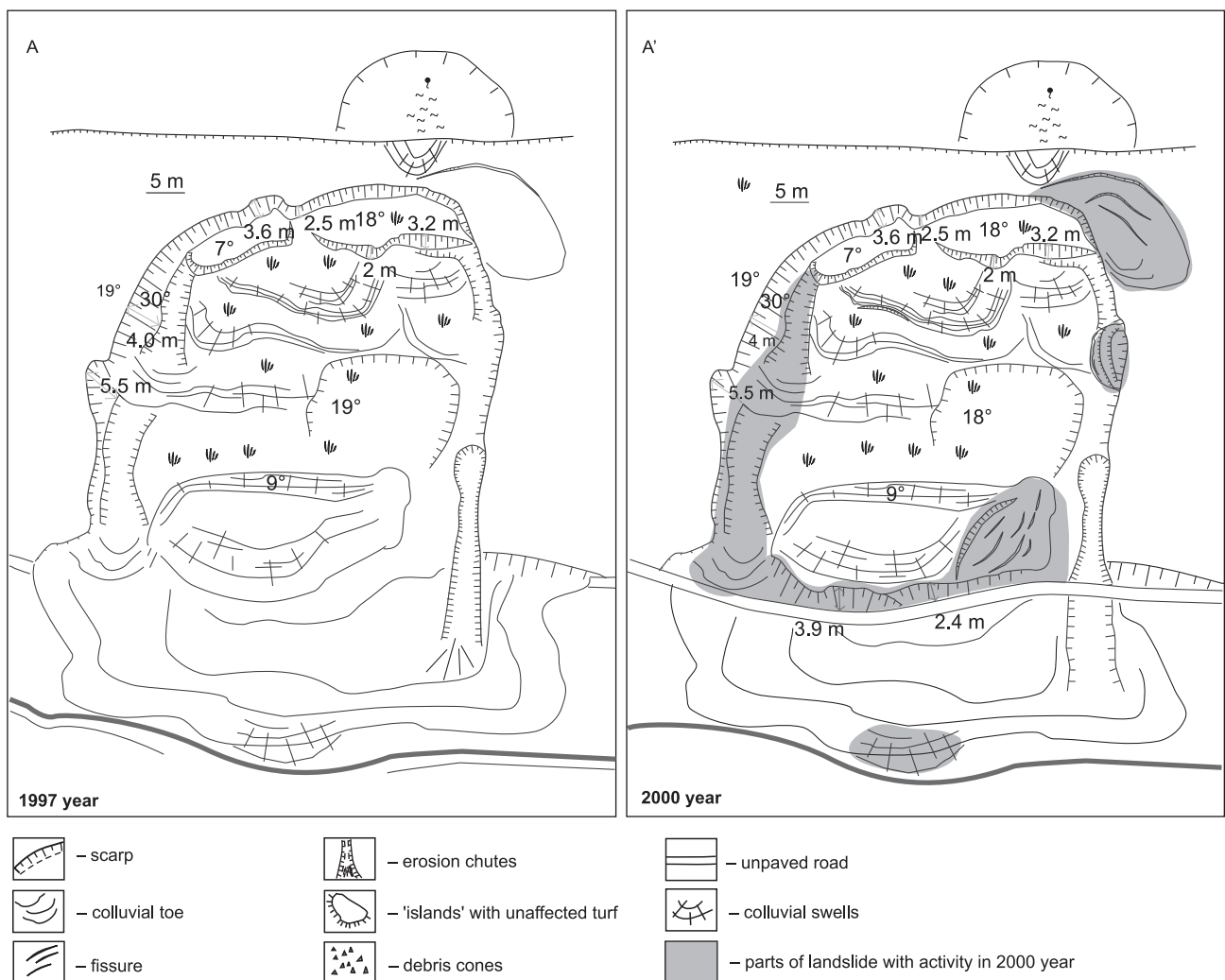
Fig. 2. A rotational slide on the slopes of the village of Mlynne (form no. 966); A – map of the slide produced in 1997 immediately after it had occurred and before human intervention; A' – map of the same slide produced in 2000
